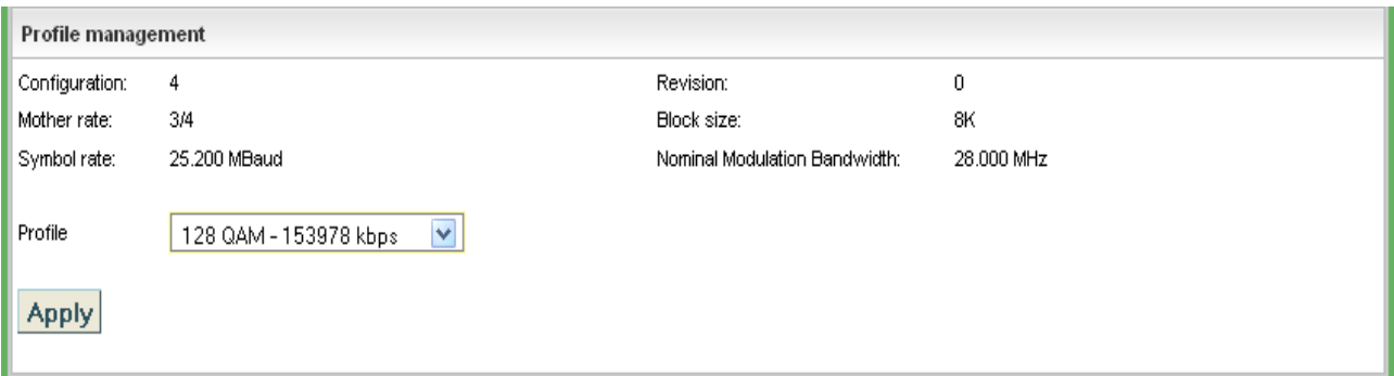
Figure 73: Web slot modem form – Profile management.
