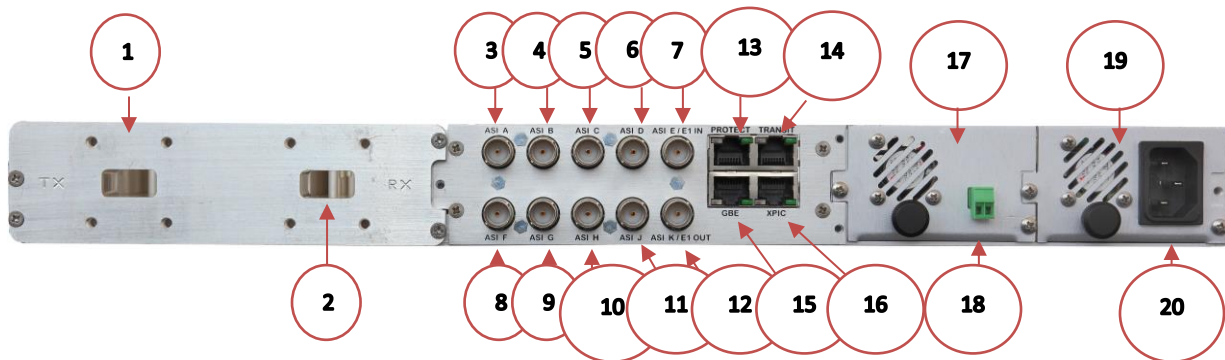
Figure 98: REBLE610 back panel.
