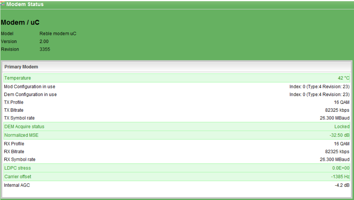
Figure 70: Web slot modem form – status.
