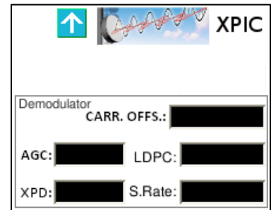
Figure 30: Modem XPIC measurements menu Rx.
