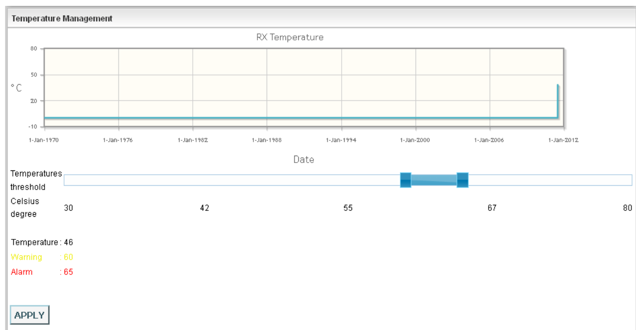
Figure 89: Web slot Rx form –Temperature Management.
